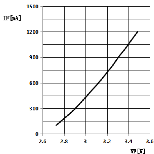
The Photoelectric Characteristics Graph (Ta= 25 °C,6000K)
